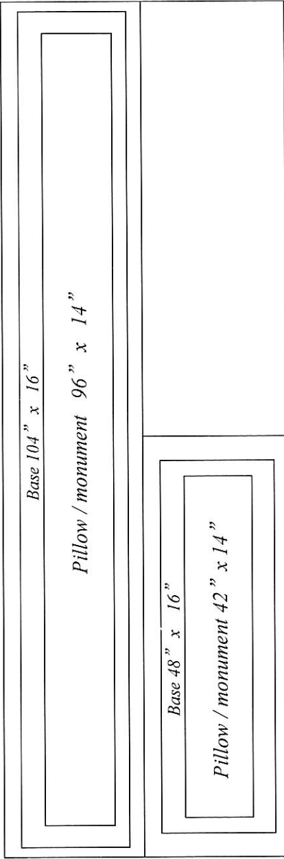
Single Cement Runner 60" x 18" Single Cement Runner 60" x 18"
